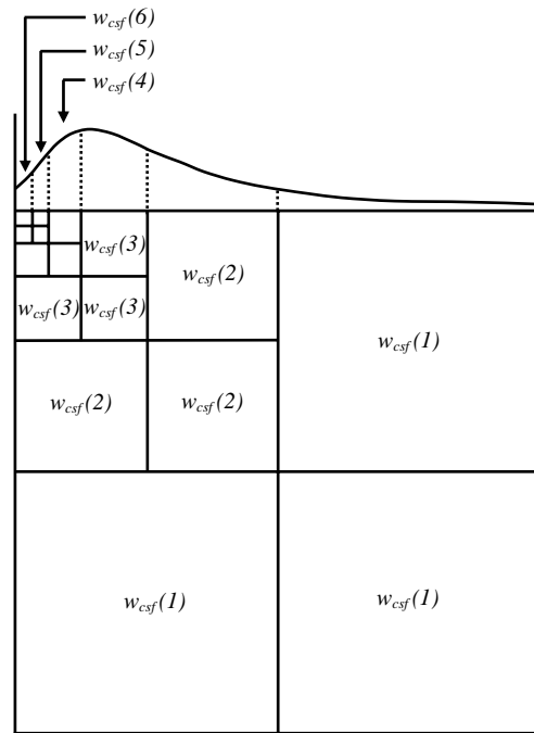
Figure 5: The matrix of quantization
