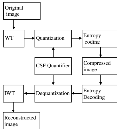
Figure 3: The incorporation of the CSF Quantifier
