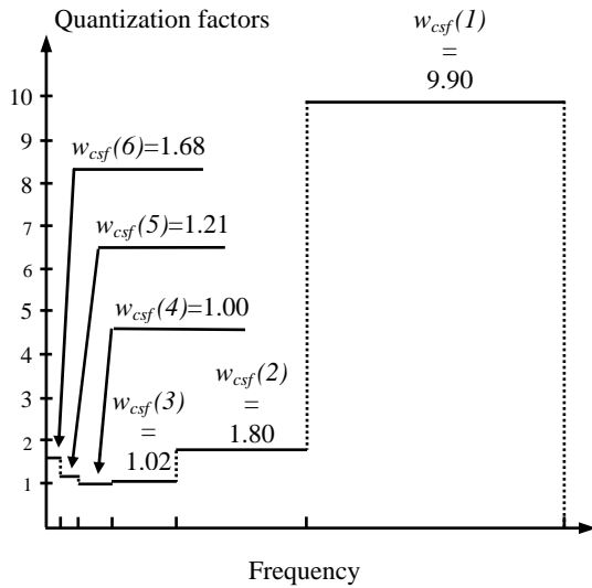
Figure 4: CSF Quantifier
